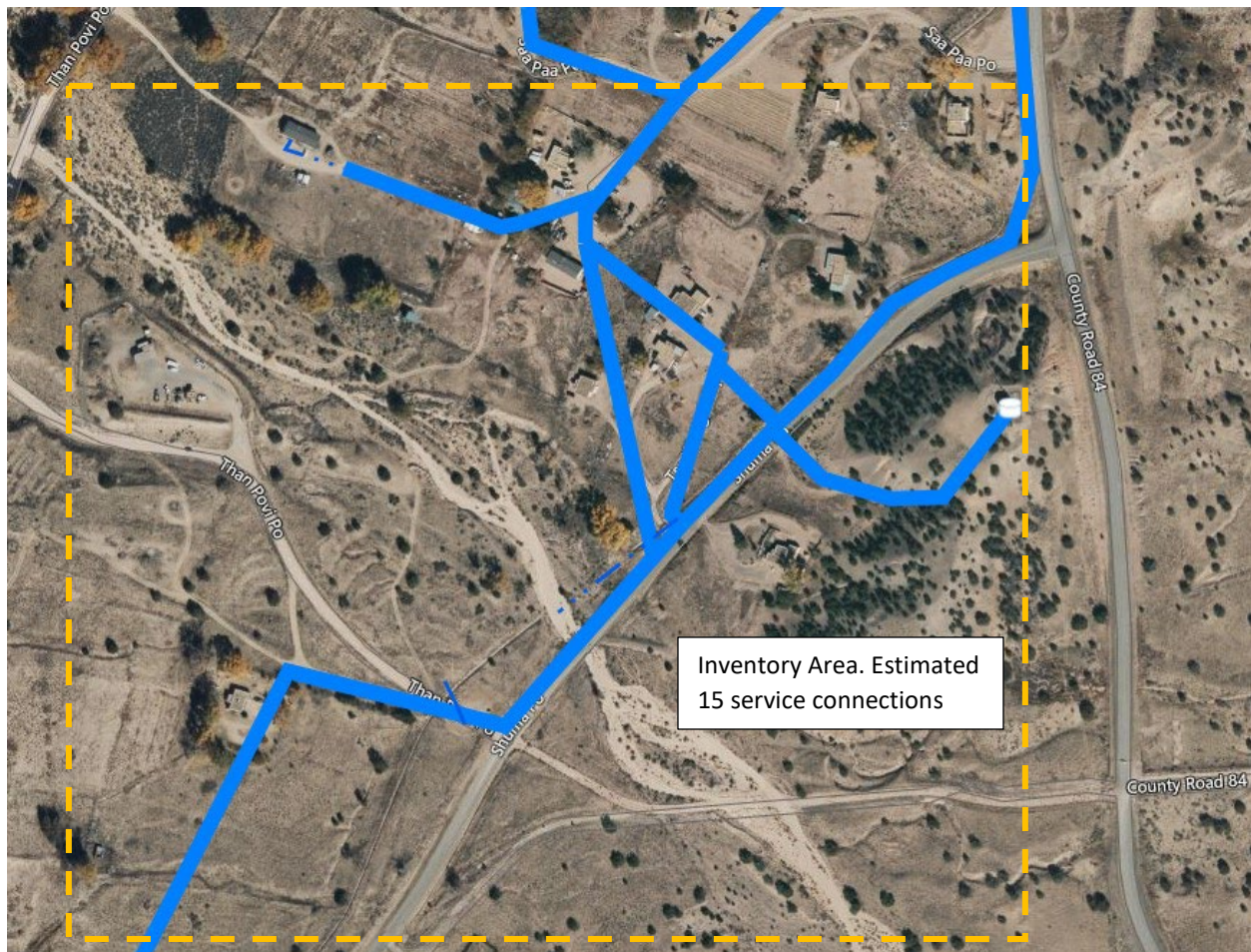
Figure 6: Tewa Tank South Service Zone
