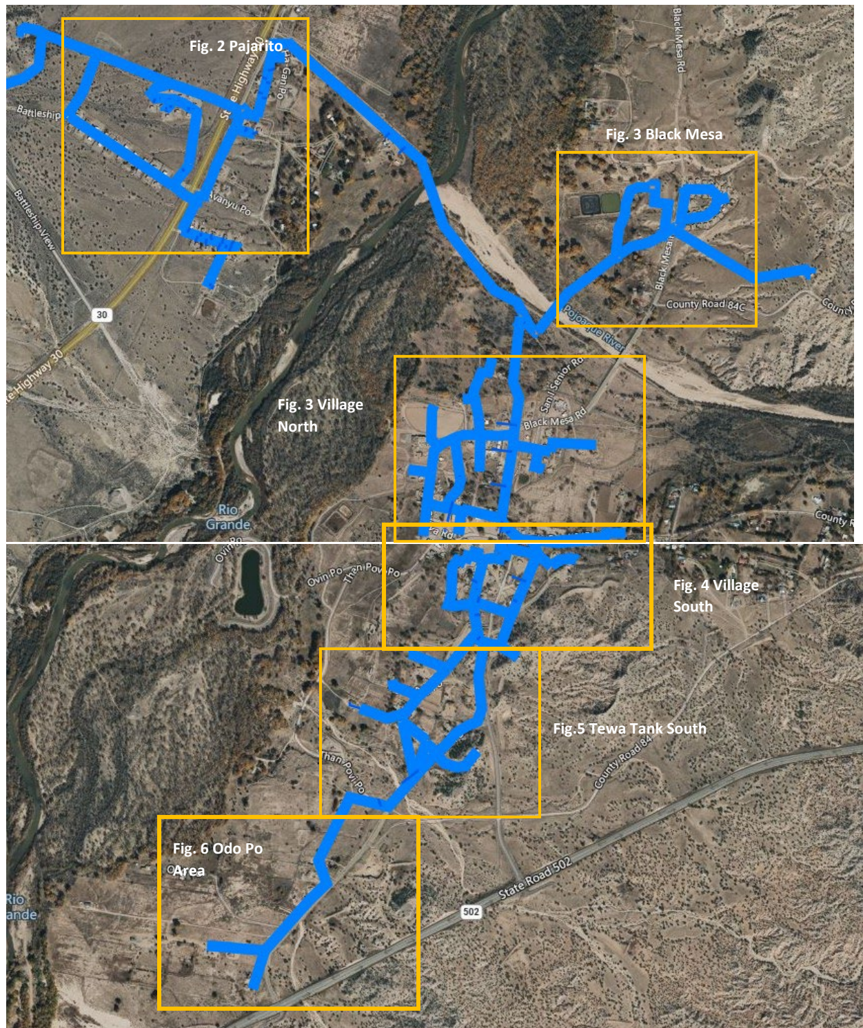
Figure 1 Overview of Service Zones
