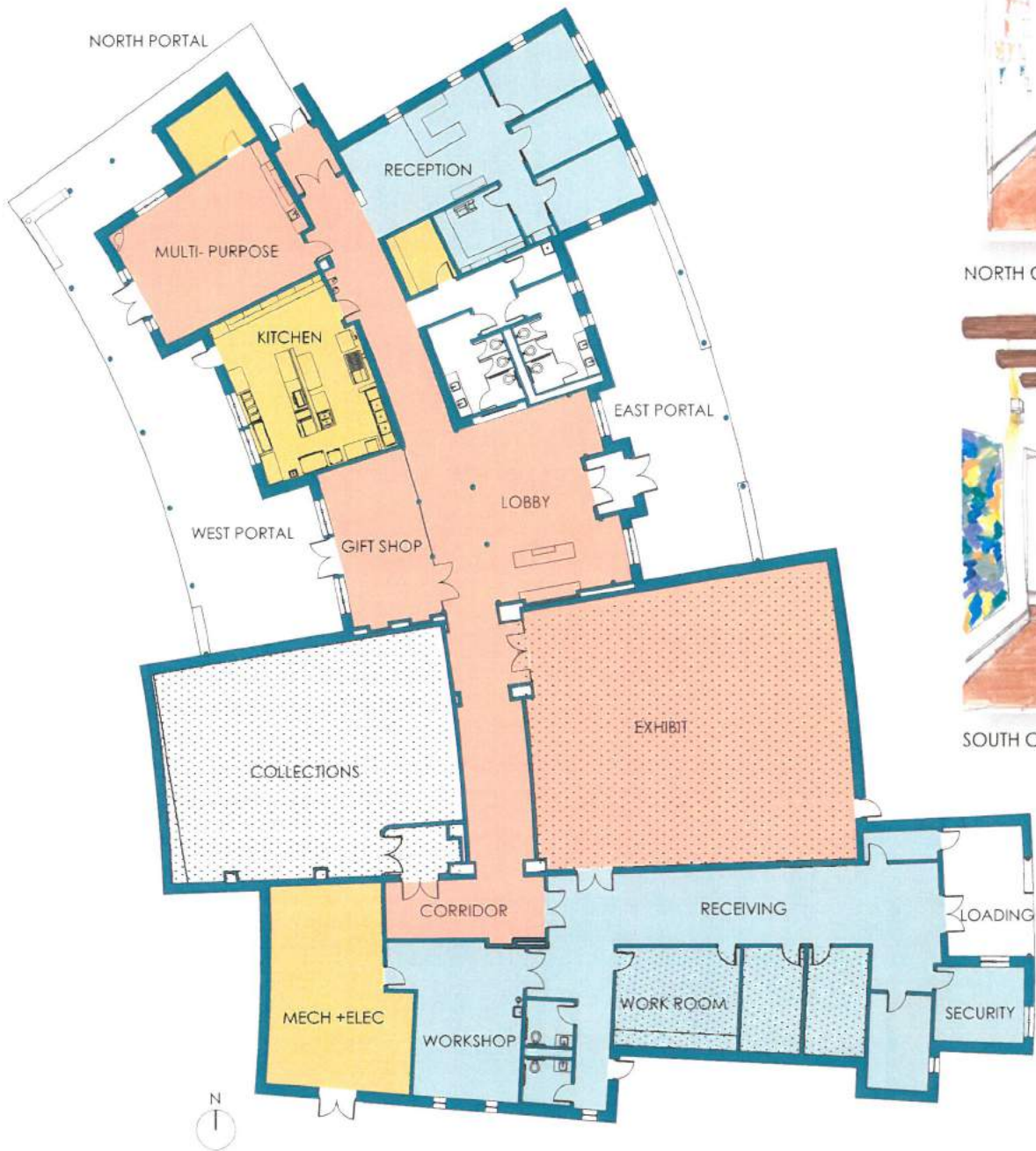
FLOOR PLAN
